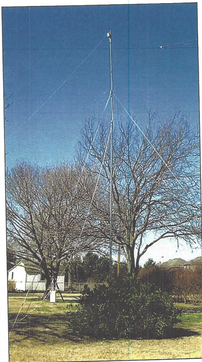
Photo A. The 40-, 20-, 15-, 10-meter off-center-fed antenna in an inverted-V configuration during testing. The apex height is 33 feet.
