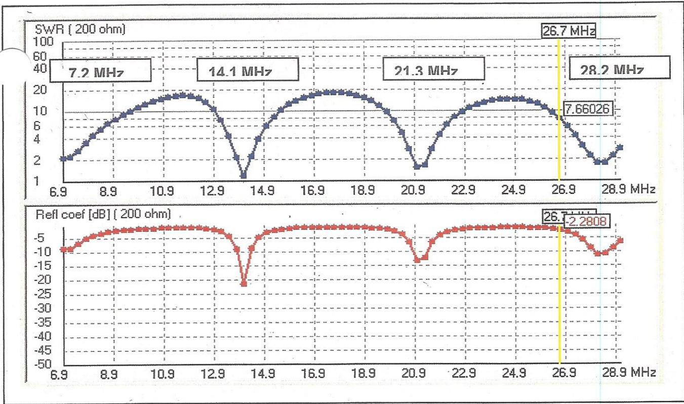
Figure 2. SWR sweep from 6.9 to 28.9 MHz for the horizontal OCF with 27-foot and 41-foot legs.
