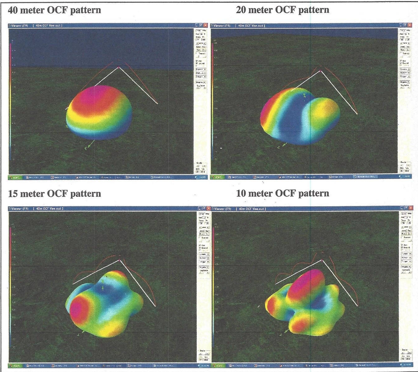
Figure 4. 3-D radiation patterns and current distributions of the OCF inverted-V antenna are shown for each band.
